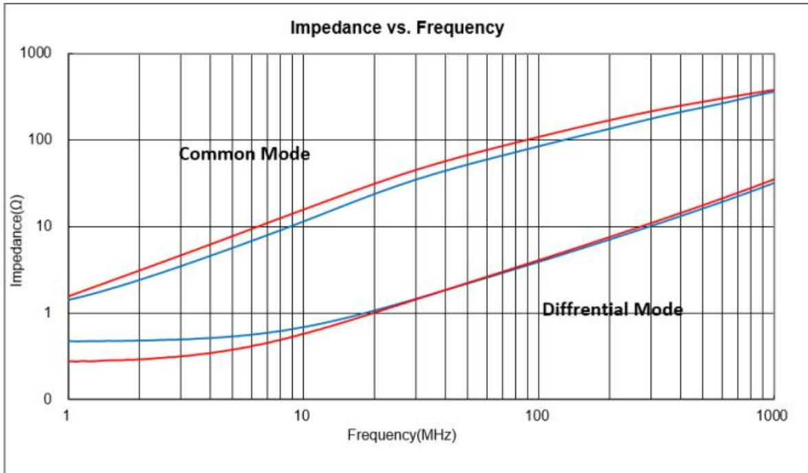
SMC0805 (90~120Ω)
